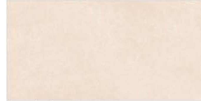
Texture Peach
